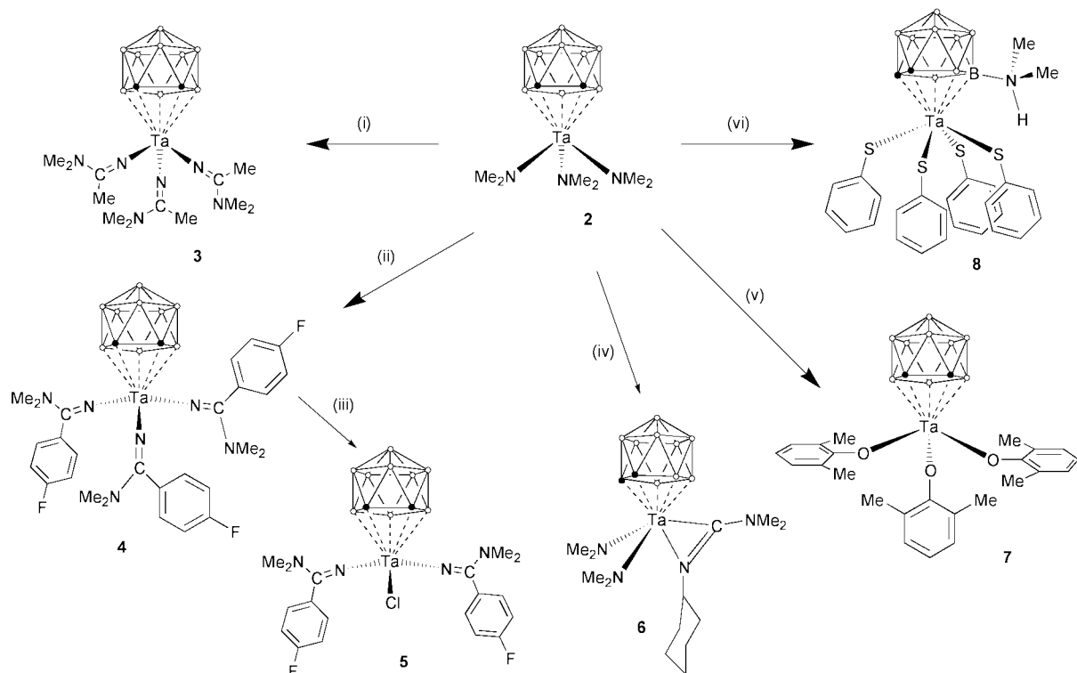
Scheme 1 The reactions of [closo-3,1,2-Ta(NMe_2)_3(C_2B_9H_{11})] , 2 , with N=C multiple bonds and with phenol and benzenethiol. Reagents: (i) acetonitrile; (ii) p -fluorobenzonitrile; (iii) CH_2Cl_2 ; (iv) cyclohexyl isocyanide; (v) 2,6-dimethylphenol; (vi) benzenethiol. Filled circles represent cluster CH, open circles cluster BH units.
