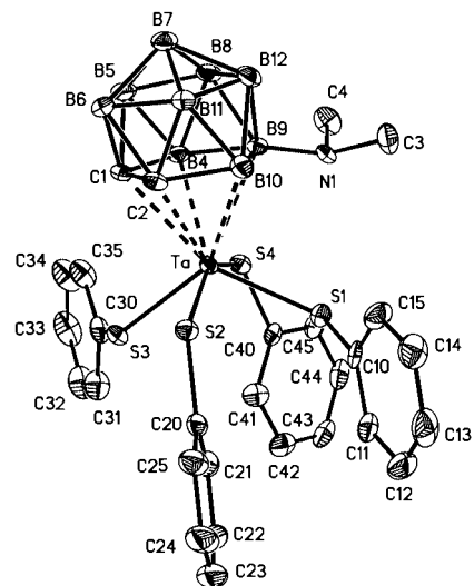
Fig. 6 The molecular structure of [ closo -3-Ta(SC 6 H 5 ) 4 (9-NHMe 2 -1,2-C 2 B 9 H 10 )], 8 . Details as in Fig. 1.
