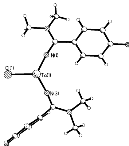
Fig. 4 A view orthogonal to the ligand plane of the Ta{N=C(C 6 H 4 F)NMe 2 }(C 2 B 9 H 11 ) 2 Cl fragment of compound 5 . Hydrogen atoms have been omitted for clarity.
